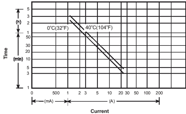
Discharge Current vs Time
