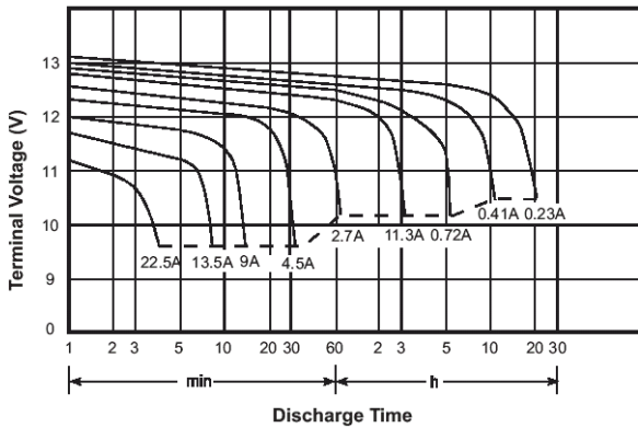
Discharge Characteristics 20 °C (68 °C)
